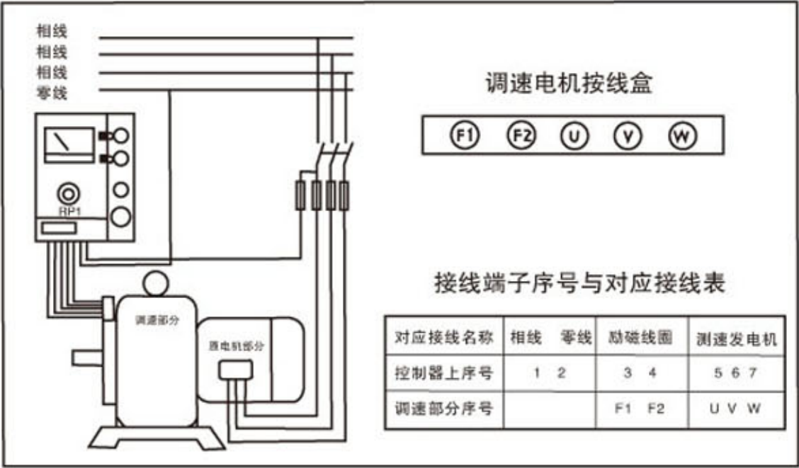
JD1A-40调速控制器与调速电机连接简图 JD1A-40 speed controller and variable-speed motor connected tube map
